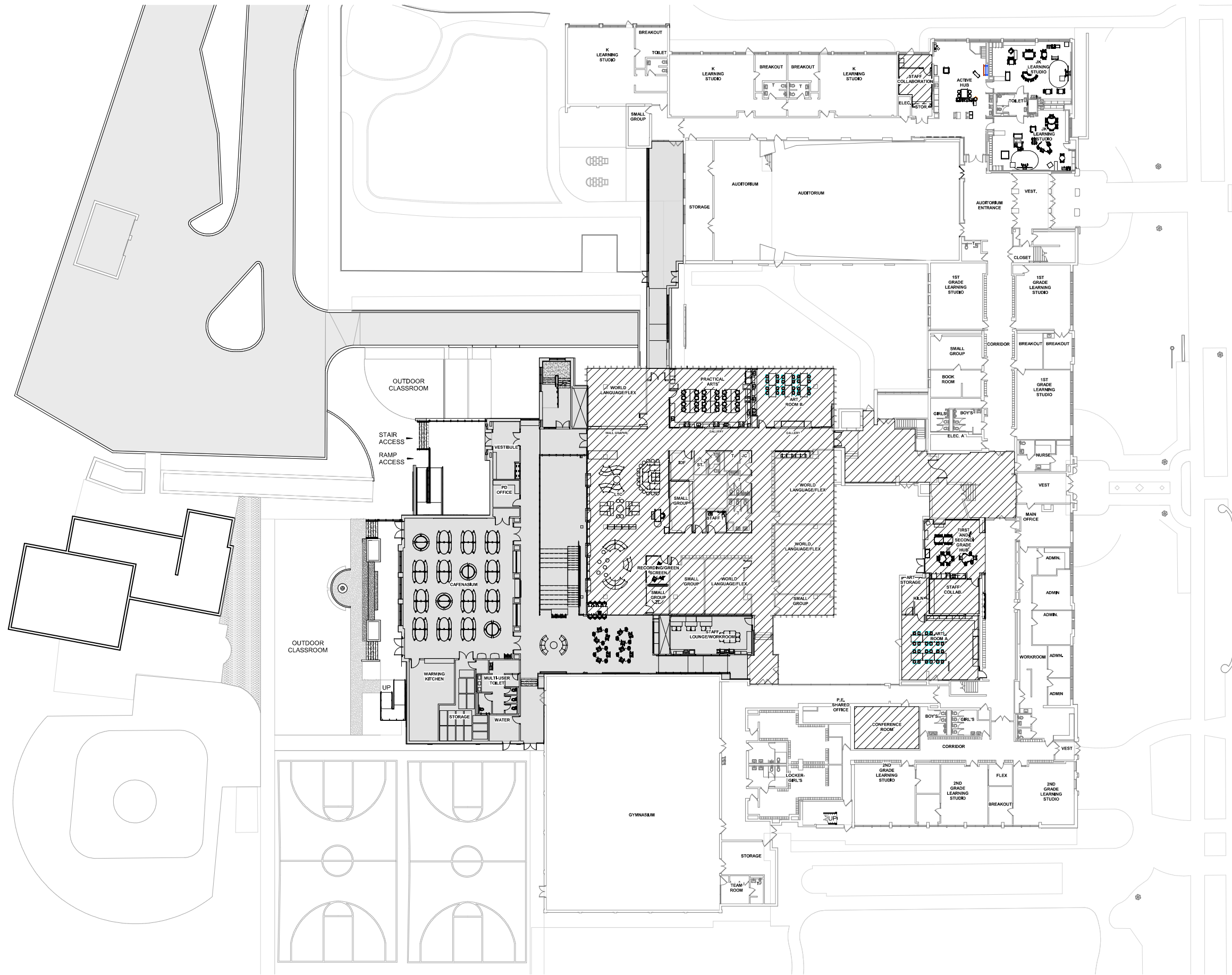
1 FIRST FLOOR MASTER PLAN 1" = 20'-0"
